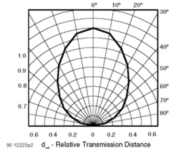
Fig. 1 - Horizontal Directivity
